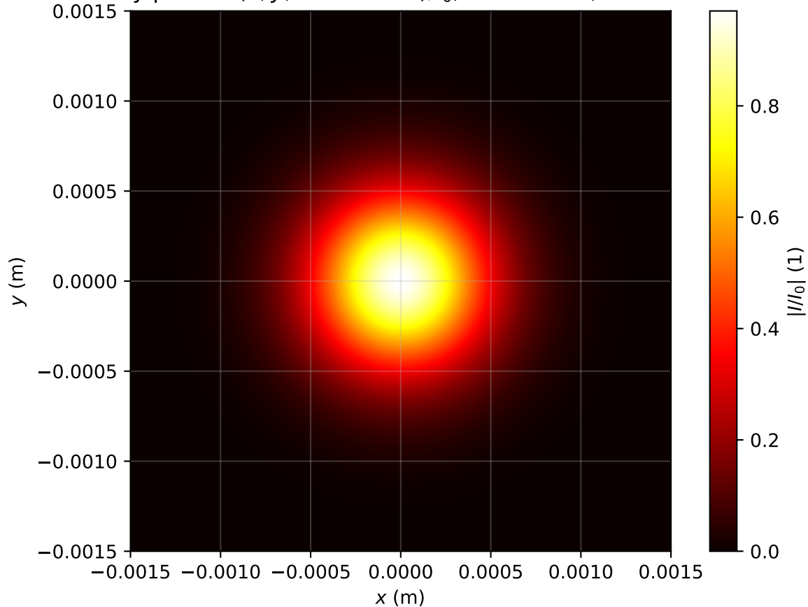
Intensity profile I(x, y, z = 0.796m)/I_0 , Pin=0.3Pcr, artificial time
